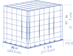
IATA ULD code: PYB Q7 Universal general-purpose flat pallet for lower holds and main decks.
