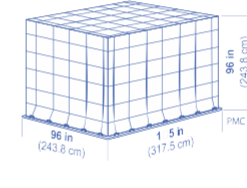
IATA ULD code: PMC Q6 Universal general-purpose flat pallet for lower holds and main decks. Tare weight: 120 kg (265 lb) Volume: H 243.8 cm (96 in), 17.0 m 3 (600 ft 3 )
