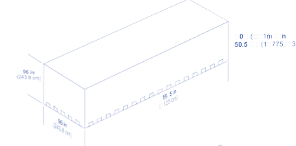
ULD code: AMA rectangular container on P6P base Main-deck container. Door is canvas with built-in net door straps. Maximum gross weight: 6,804 kg (15,000 lb) Tare weight: 350 kg (772 lb)
